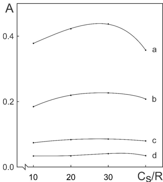
Figure 3 - Effect of the C_s/R flow rates ratio on the signal response for 10.00 (a), 5.00 (b), 2.00 (c) and 1.00 (d) \mu\text{g/L} Hg.
